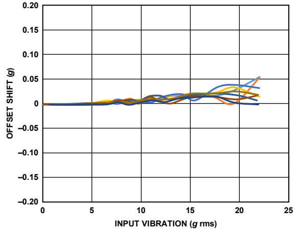
Figure 48. ADXL357 VRE, Y-Axis Offset from -1 g, \pm 40 g Range, Y-Axis Orientation = -1 g
