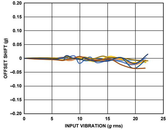
Figure 49. ADXL357 VRE, Z-Axis Offset from +1 g, \pm 40 g Range, Z-Axis Orientation = +1 g
